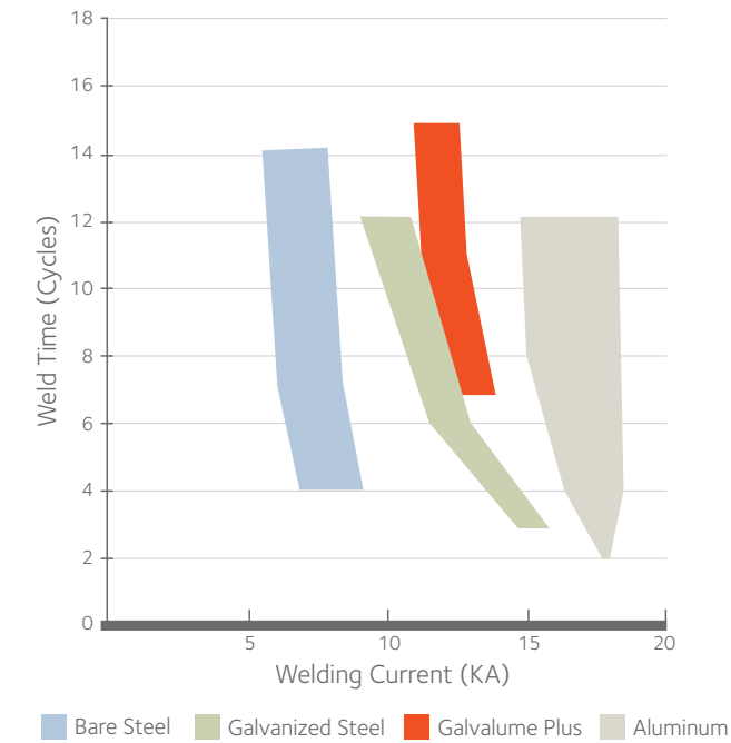
Welding Lobes for Various Steel Sheets and Aluminum
