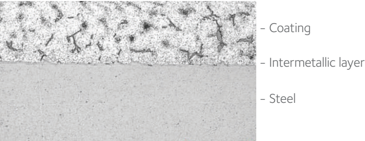
Galvalume Coating Metallographic Cross-Section (500x)
