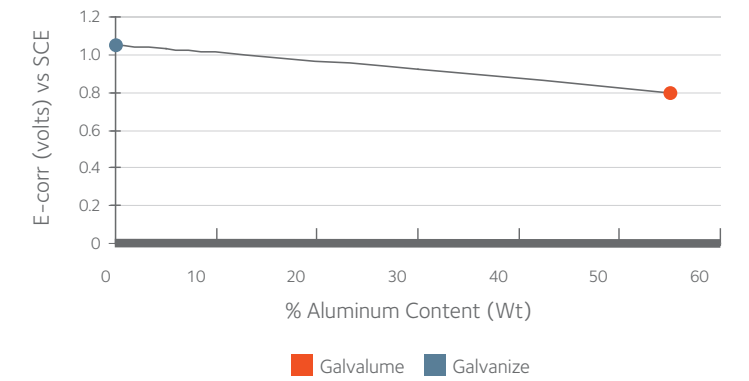
Corrosion Potential After 3 Years Atmospheric Exposure
